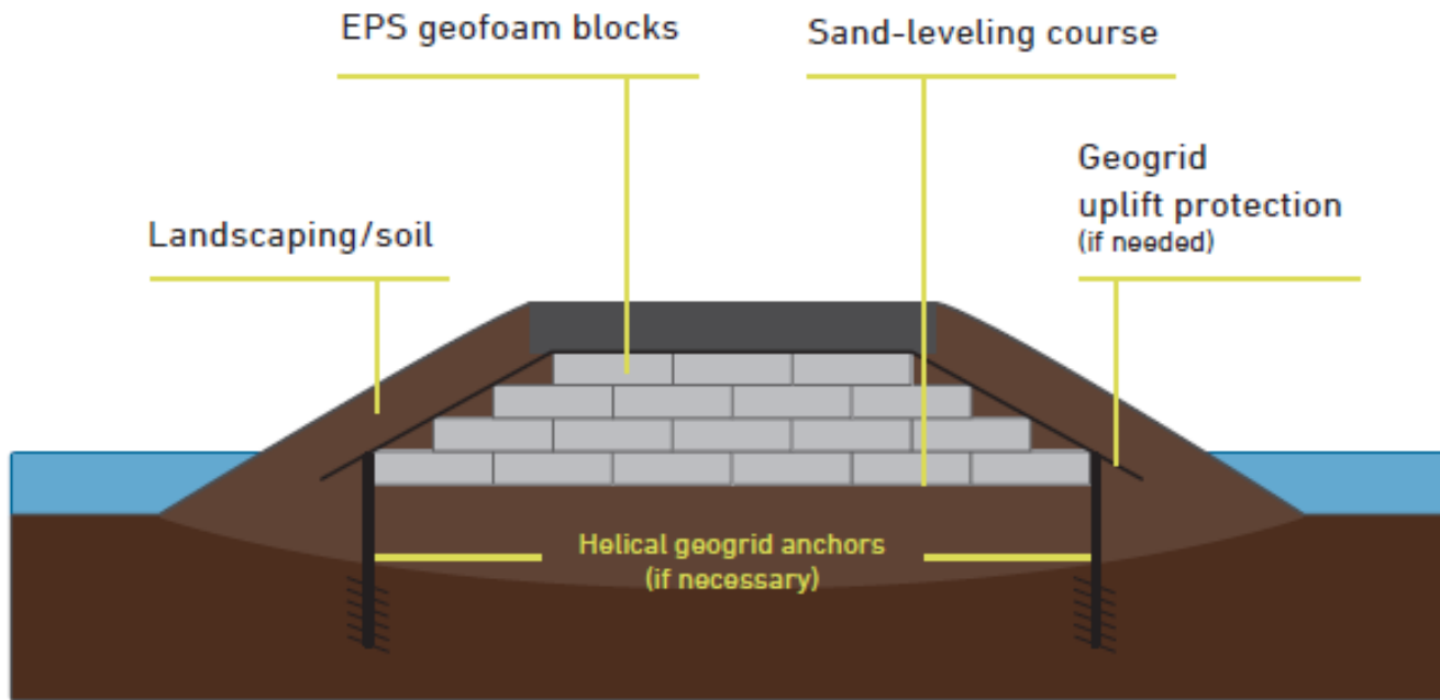
Schematic drawing of levee repair using EPS geofoam
